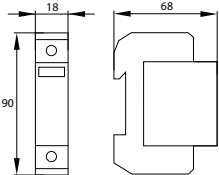
▶ SPD01/02-1P
